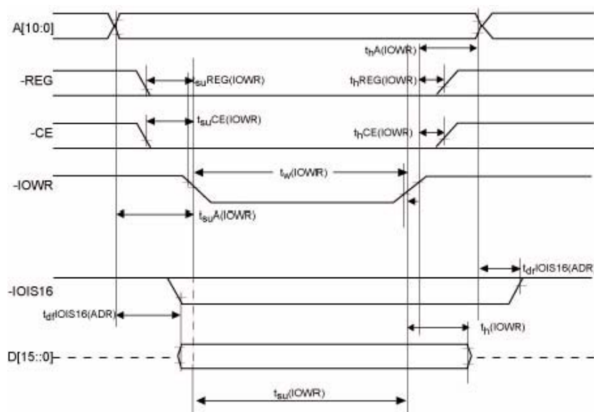
Figure 8: I/O Write Timing Diagram
