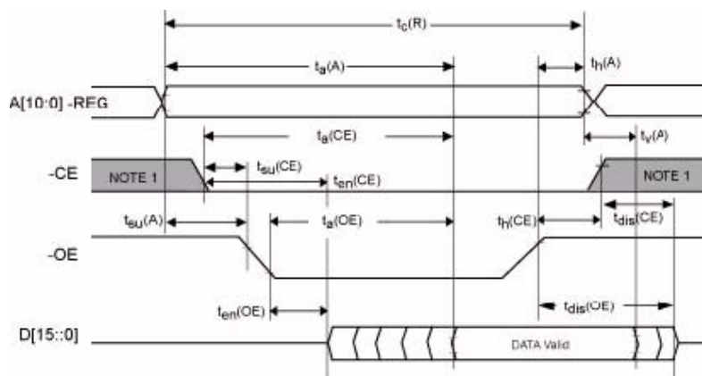
Figure 5: Common and Attribute Memory Read Timing Diagram
