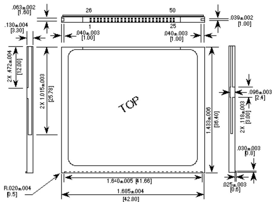
Figure 2: CompactFlash 5000 Dimensions
