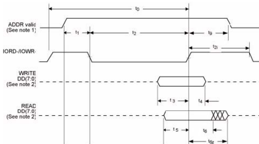
Figure 9: Register Transfer to/from Device
