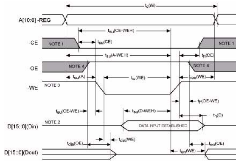
Figure 6: Common and Attribute Memory Write Timing Diagram
