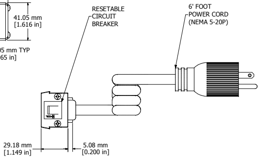
ASSEMBLY - VIEW FROM END
