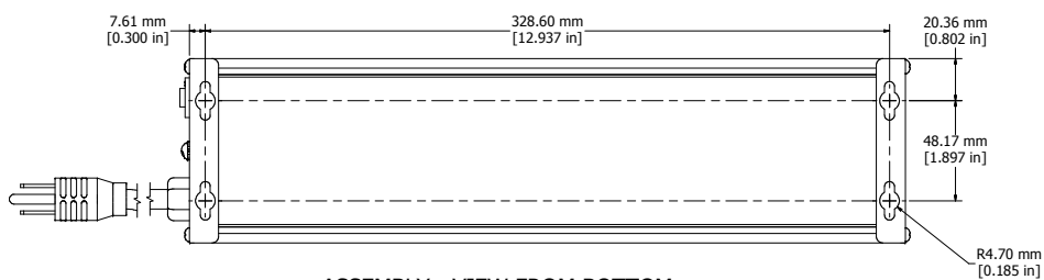
ASSEMBLY - VIEW FROM BOTTOM
