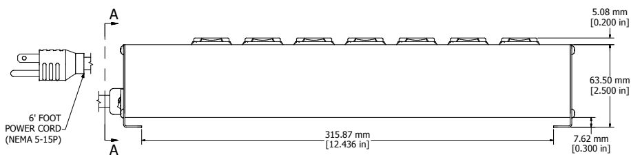
ASSEMBLY - VIEW FROM SIDE
