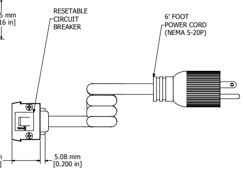
ASSEMBLY - VIEW FROM END
