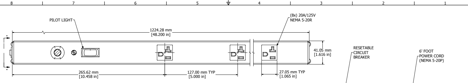
SECTION A-A (VIEW FROM FRONT)
