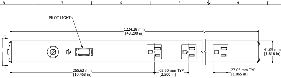
SECTION A-A (VIEW FROM FRONT)
