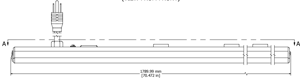
ASSEMBLY - VIEW FROM SIDE
