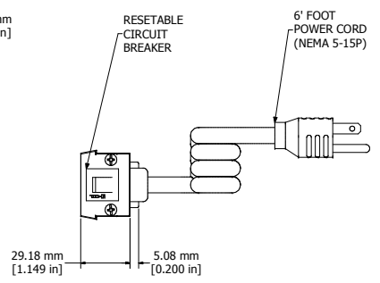
ASSEMBLY - VIEW FROM END
