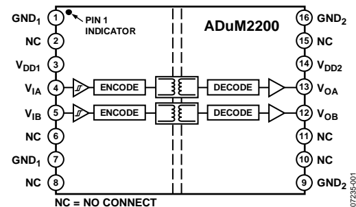
Figure 1. ADuM2200
