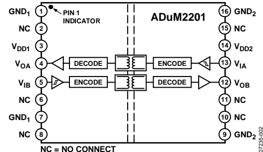
Figure 2. ADuM2201
