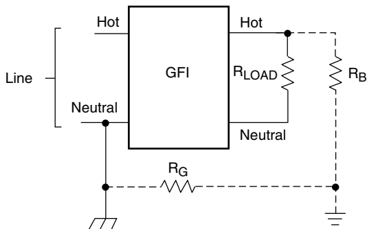
Figure 1. Normal Fault
