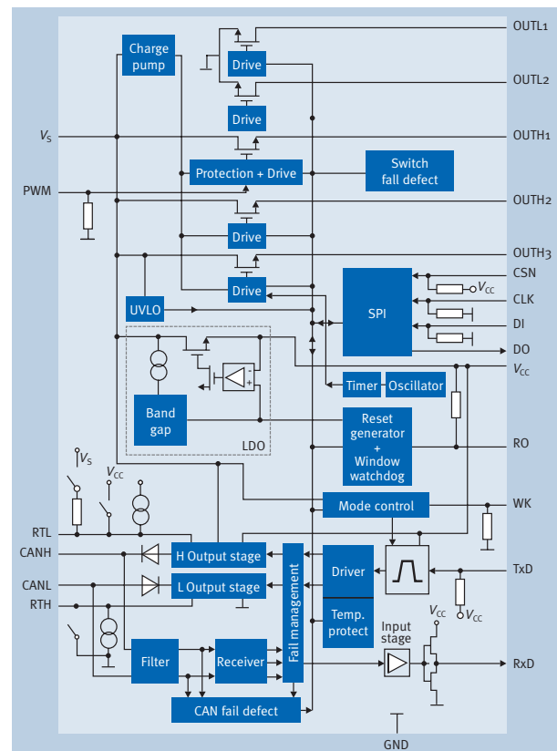
Block diagram TLE6266G
