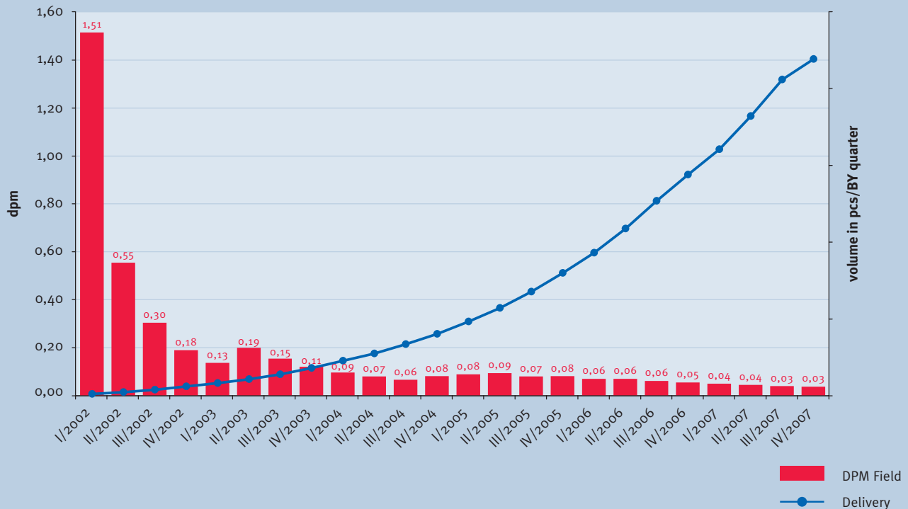
Average failure (ppm) for TLE6250G
