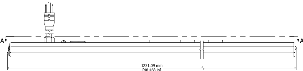
ASSEMBLY - VIEW FROM SIDE
