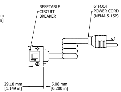
ASSEMBLY - VIEW FROM END
