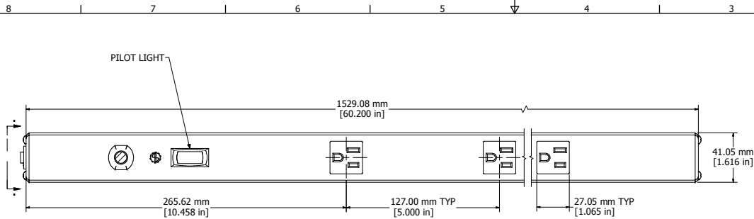
SECTION A-A (VIEW FROM FRONT)
