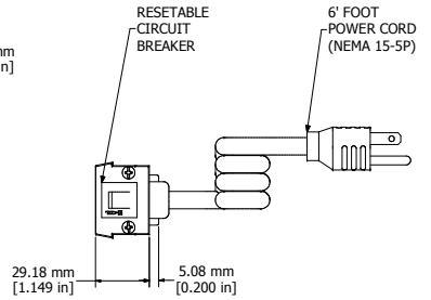
ASSEMBLY - VIEW FROM END
