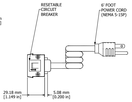
ASSEMBLY - VIEW FROM END
