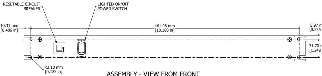
ASSEMBLY - VIEW FROM FRONT
