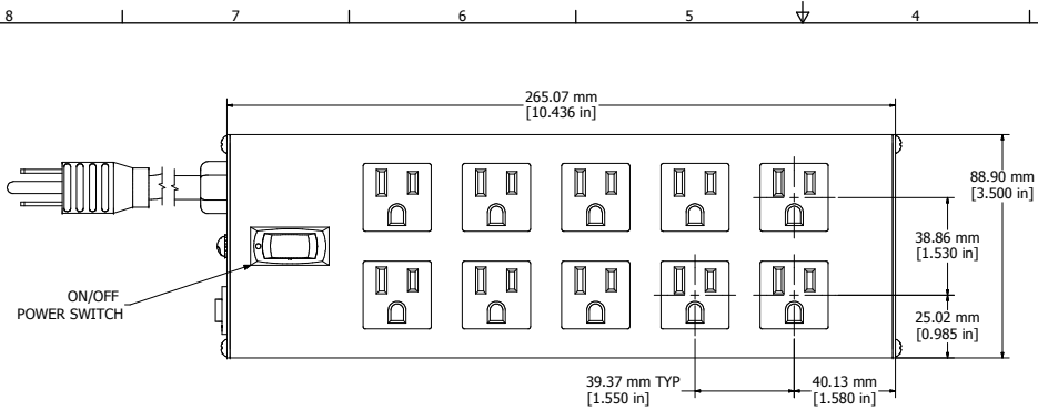
ASSEMBLY - VIEW FROM TOP
