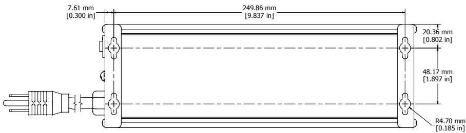
ASSEMBLY - VIEW FROM BOTTOM
