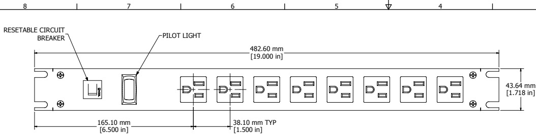
ASSEMBLY - VIEW FROM FRONT
