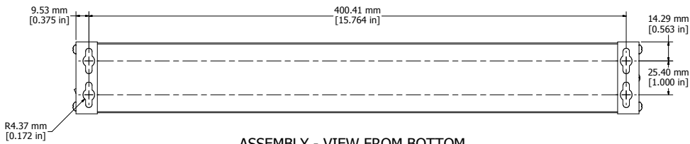
ASSEMBLY - VIEW FROM BOTTOM
