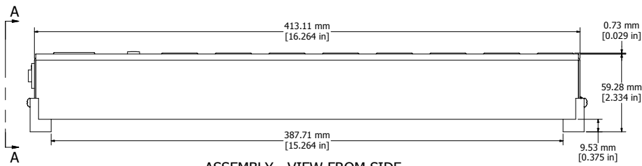
ASSEMBLY - VIEW FROM SIDE
