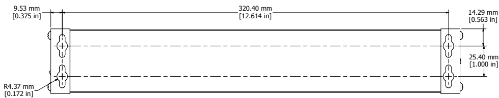
ASSEMBLY - VIEW FROM BOTTOM
