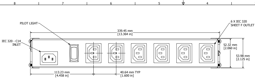
ASSEMBLY - VIEW FROM TOP
