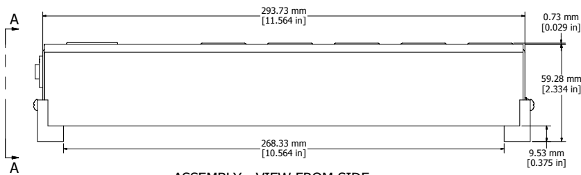
ASSEMBLY - VIEW FROM SIDE
