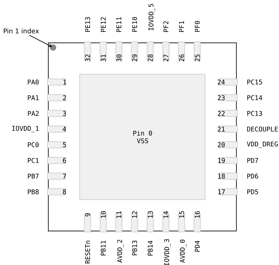
Figure 4.1. EFM32G210 Pinout (top view, not to scale)
