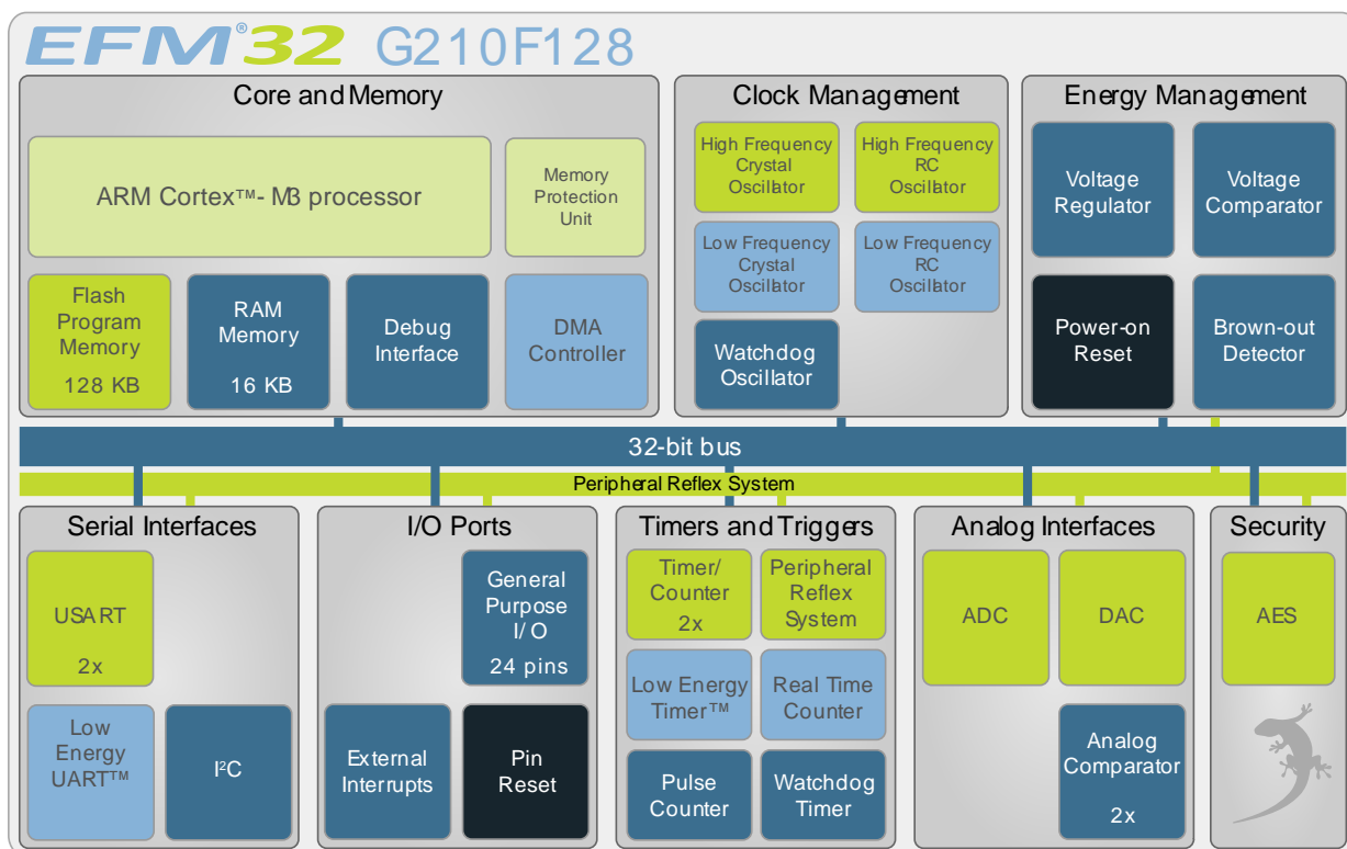
Figure 1.1. Block Diagram
