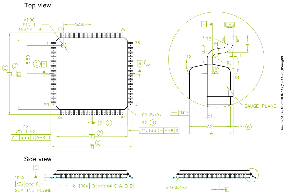
Figure 4.2. LQFP100
