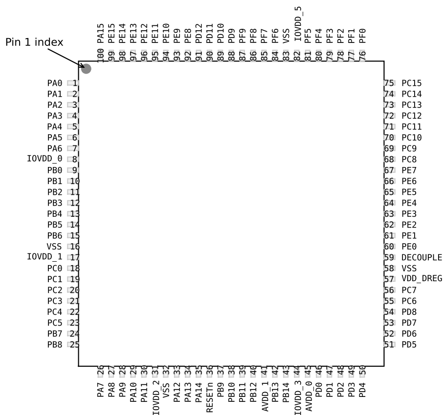
Figure 4.1. EFM32G280 Pinout (top view, not to scale)
