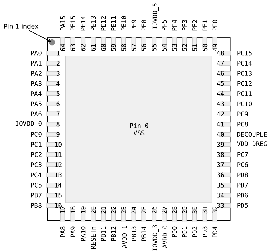
Figure 4.1. EFM32G230 Pinout (top view, not to scale)
