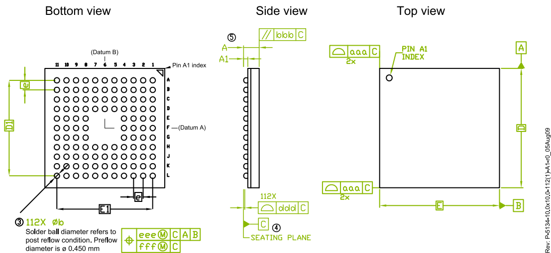
Figure 4.2. BGA112
