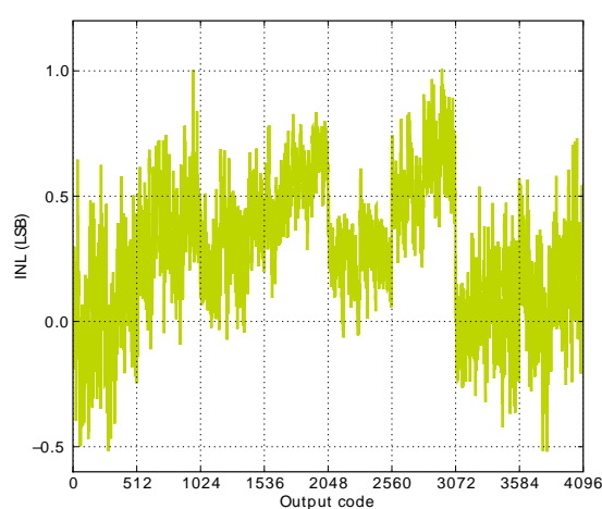
5VDIFF Reference
