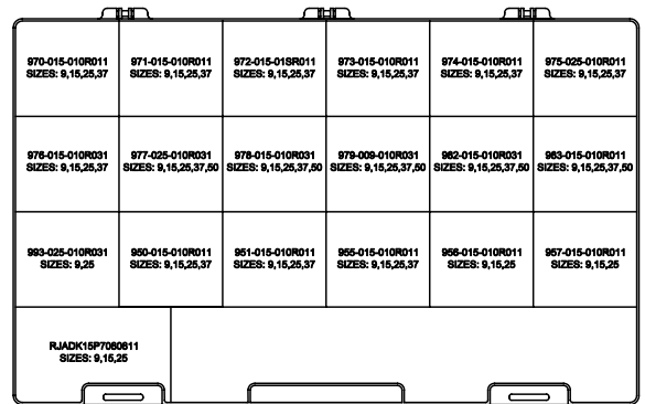
INSIDE VIEW
