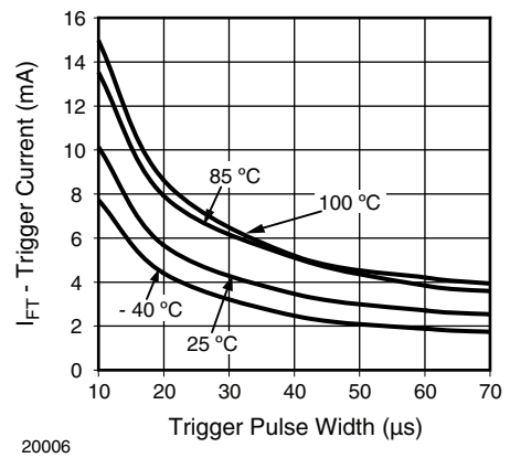
Fig. 1 I_{FT} vs. LED Pulse Width
