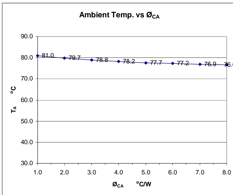
Figure 3 89TTM553 Ambient Temperature Curve
