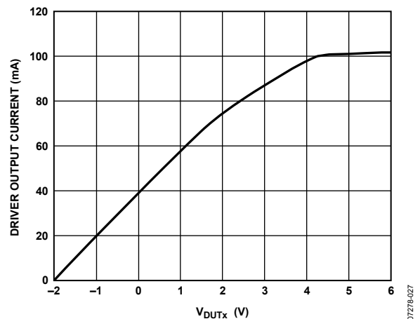
Figure 27. Driver Output Current Limit; Driver Programmed to -2.0 V; V DUTx Swept from -2.0 V to +6.0 V
