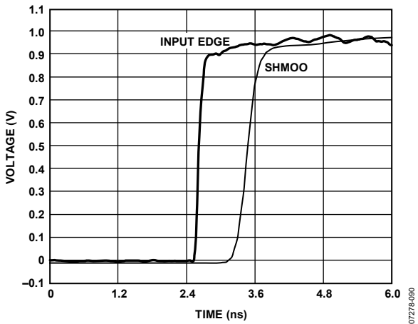
Figure 35. Comparator Shmoo; 1.0 V Swing; 200 ps (10%/90%)
