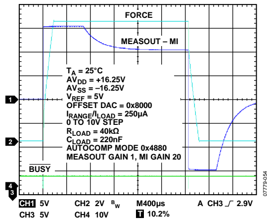
Figure 39. Transient Response FVMI Mode, ±250 µA Range, Autocompensation Mode
