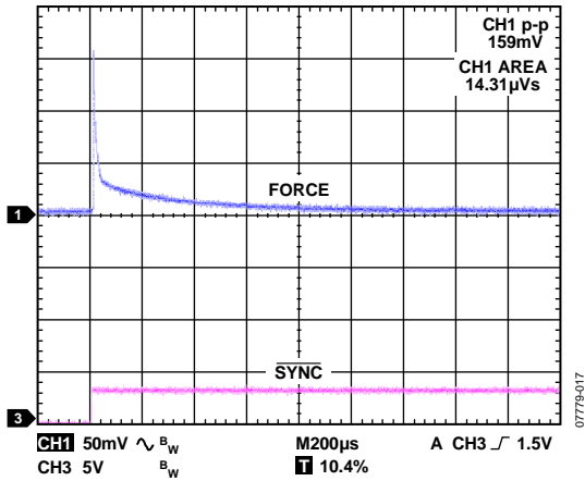
Figure 31. Range Change 25 mA to EXTFORCE2, Safe Mode, 25 mA I_{LOAD} , 10 \mu F Load
