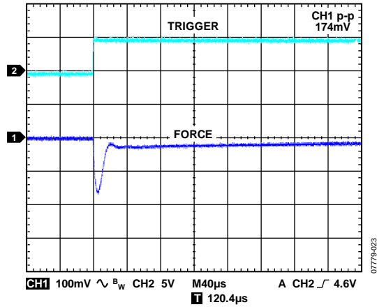
Figure 37. Safe Mode 10% to 90%, EXTFORCE2 Range, 10 µF Load
