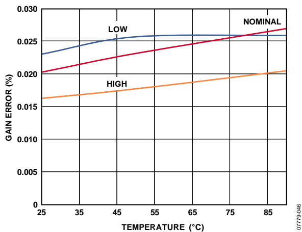
Figure 27. MV Gain Error vs. Temperature, MEASOUT Gain = 0.2
