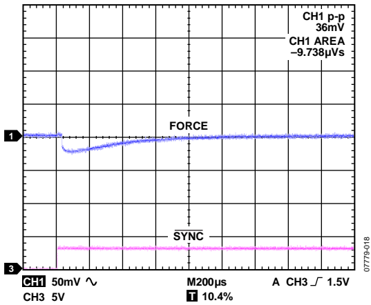
Figure 32. Range Change EXTFORCE2 to 25 mA, Safe Mode, 25 mA I_{LOAD} , 10 \mu F Load
