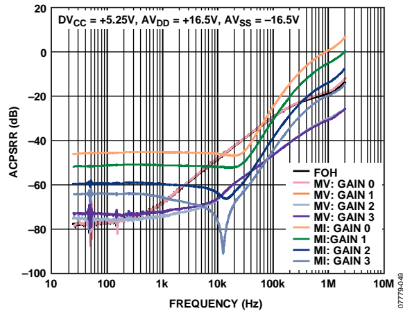
Figure 47. ACPSRR of AVDD vs. Frequency
