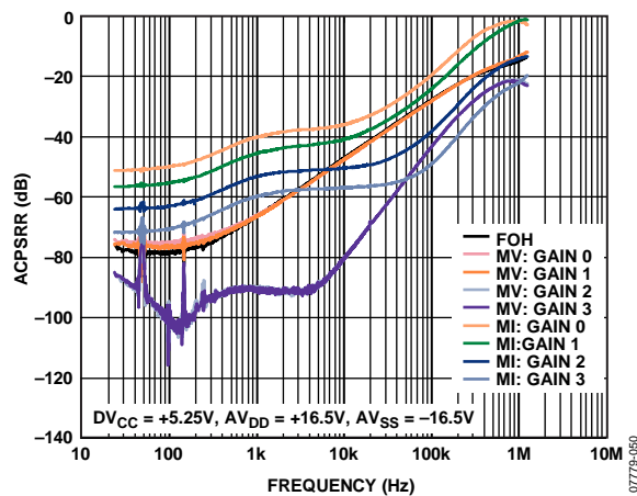
Figure 48. ACPSRR of AVSS vs. Frequency
