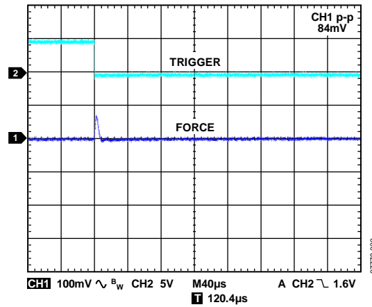
Figure 34. Autocompensation Mode 90% to 10% I_{LOAD} Change, EXTFORCE2 Range, 10 \mu F Load
