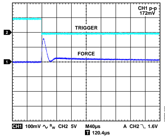
Figure 36. Safe Mode 80% to 10% I_{LOAD} Change, EXTFORCE2 Range, 10 \mu F Load
