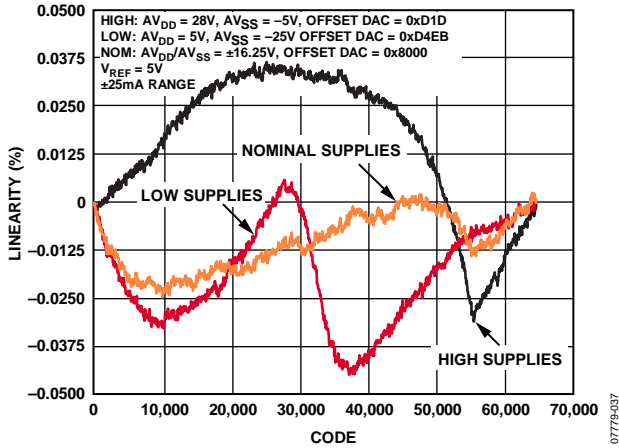
Figure 13. Measure Current Linearity vs. Code (MEASOUT Gain = 0.2, MI Gain = 20)
