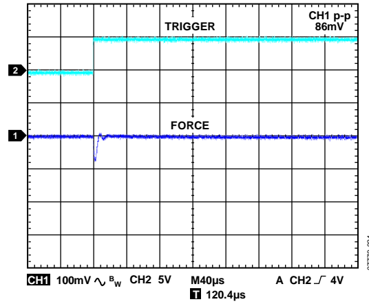
Figure 35. Autocompensation Mode 10% to 90% I_{LOAD} Change, EXTFORCE2 Range, 10 \mu F Load
