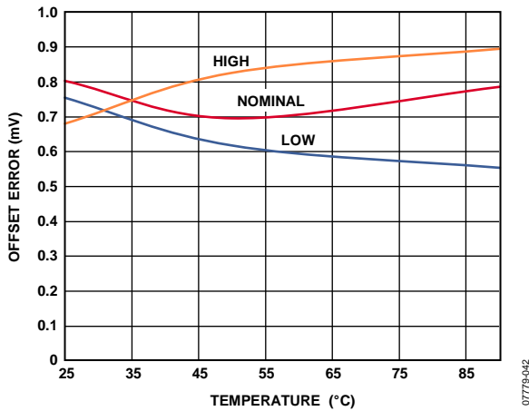
Figure 26. MV Offset Error vs. Temperature, MEASOUT Gain = 1
