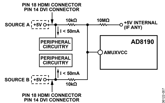
Figure 28. Suggested AMUXVCC Power Scheme
