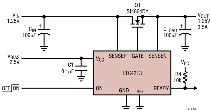
Figure 1. LTC4213 Electronic Circuit Breaker Application
