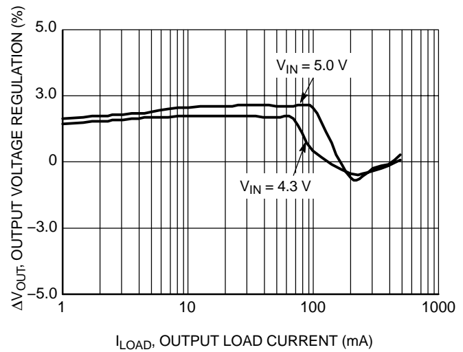
Figure 26. Output Voltage Regulation vs. Output Load Current ( V_{OUT} = 3.3\text{ V} )
