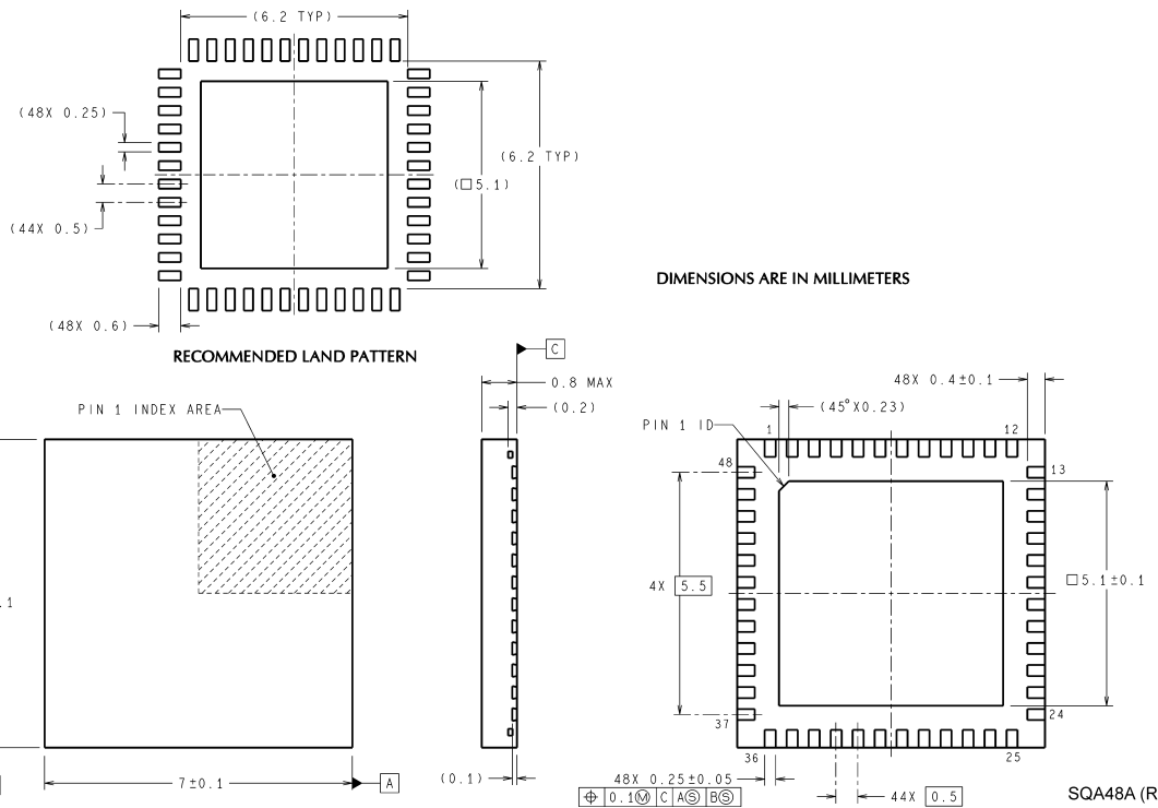
48-Lead LLP Package Order Number LM27212SQ NS Package Number SQA48A
