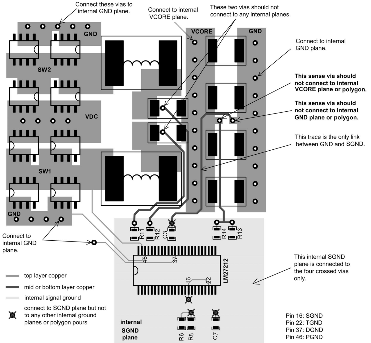
FIGURE 2. PCB Layout Example
