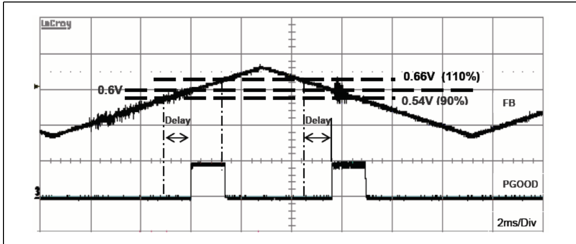
Figure 11. PGOOD signal
