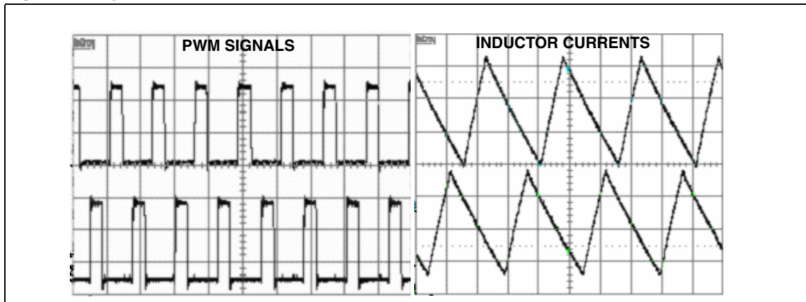
Figure 21. Synchronization.
