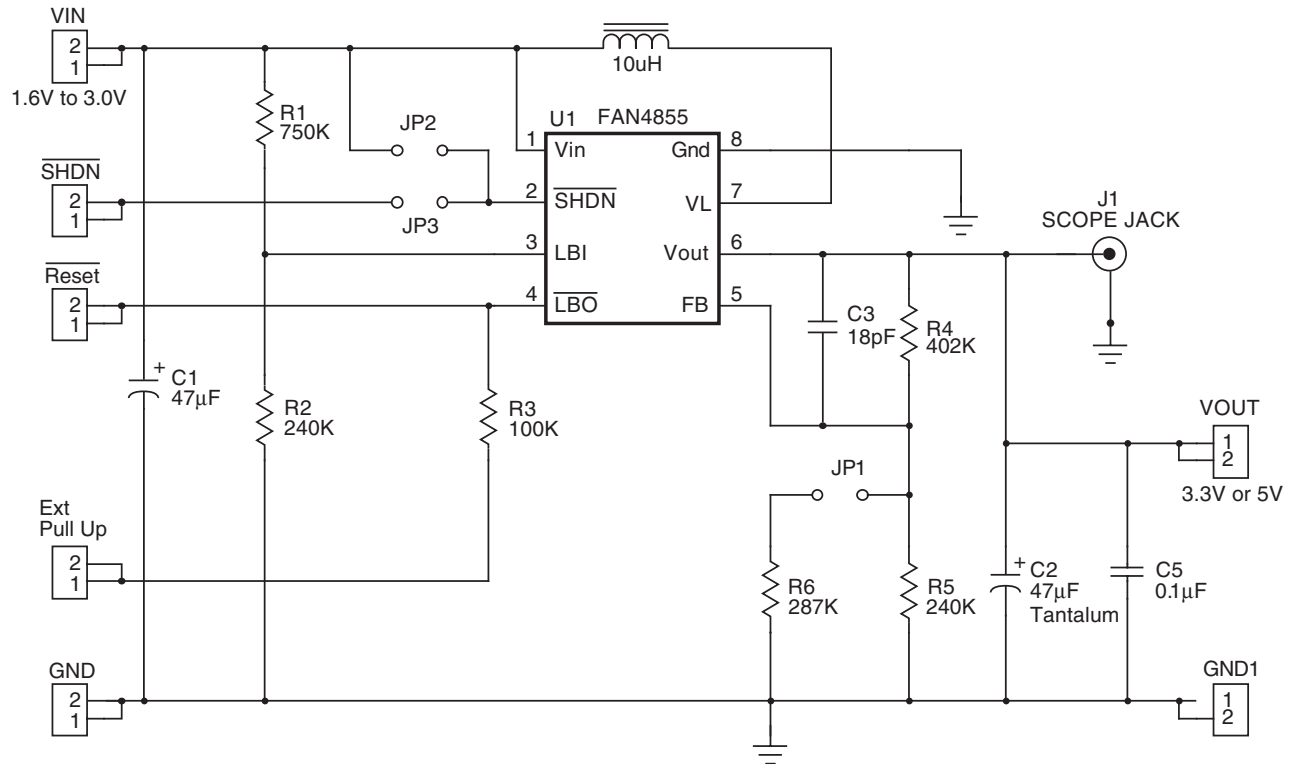
Figure 1. Test Circuit
