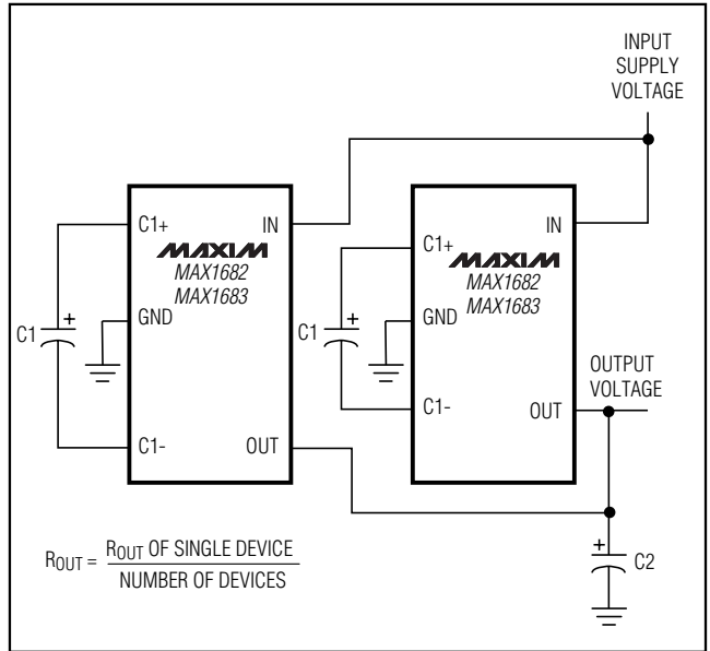
Figure 4. Paralleling Devices
