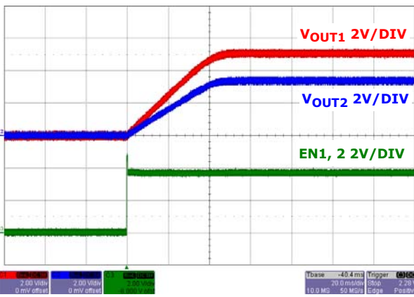
FIGURE 30. RATIOMETRIC START-UP SEQUENCING AT NO LOAD
