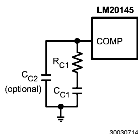
FIGURE 5. Compensation Network for LM20145
