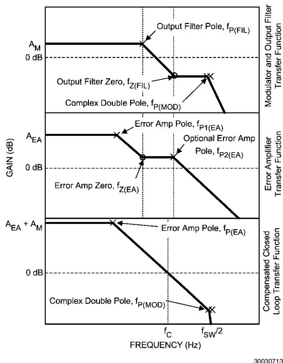
FIGURE 4. LM20145 Loop Compensation
