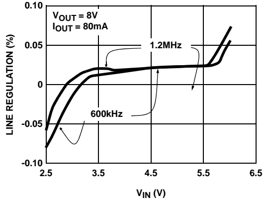
FIGURE 16. LINE REGULATION
