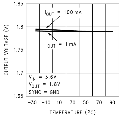
Output Voltage vs Temperature ( V_{OUT}= 1.8V , PFM Mode)
