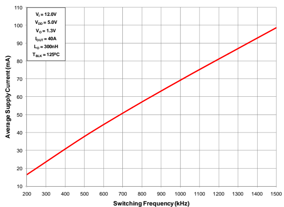
Figure 8 V DD supply current vs. Frequency
