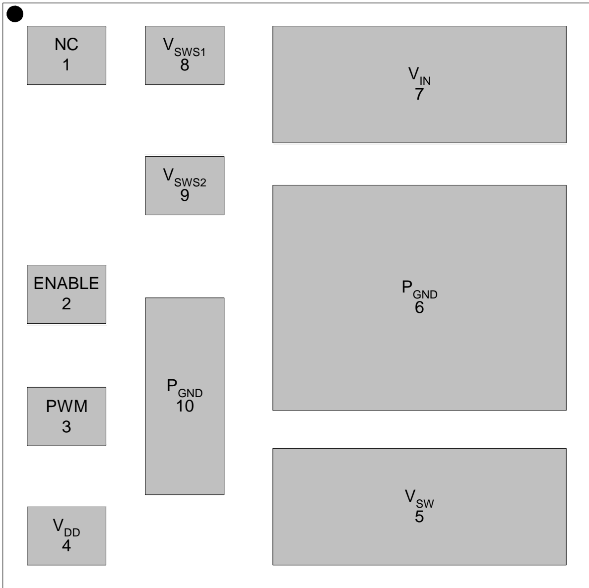
Figure 13 Top Side Transparent View
