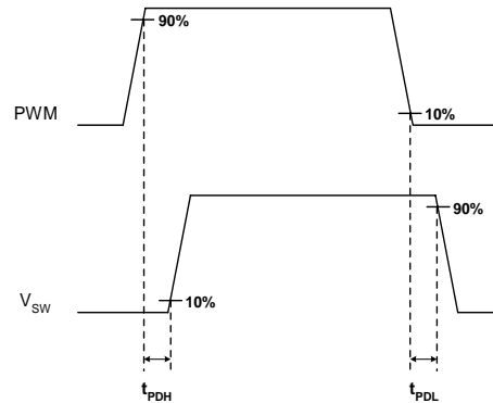
Figure 10 Timing Diagram
