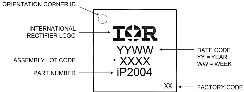
Figure 19 Part Marking
