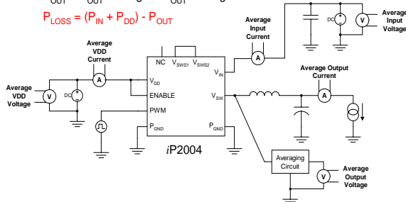
Figure 9 Power Loss Test Circuit
