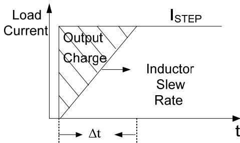
Figure 18. Charge Requirement during Load Step
