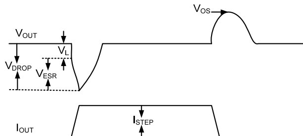
Figure 19. Typical Output Voltage Response Waveform.
