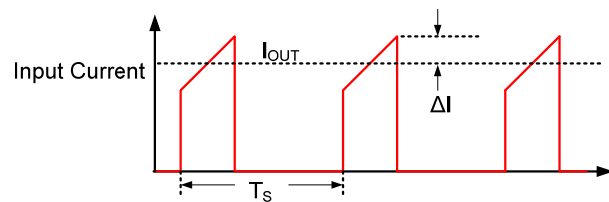
Figure 17. Typical Input Current Waveform.
