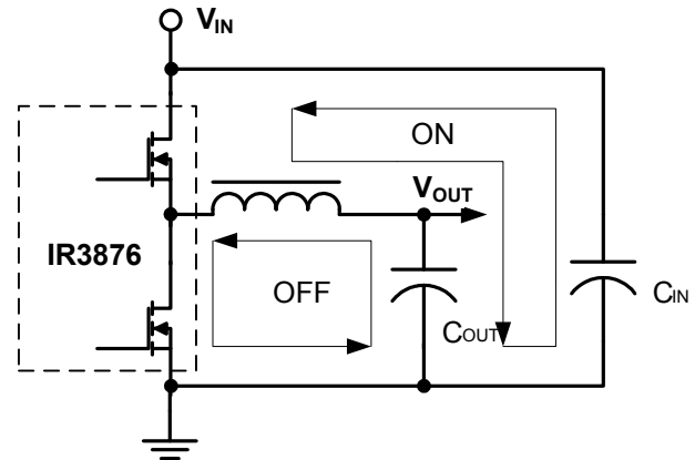
Figure 20. Current Path of Power Stage
