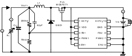
Circuit
