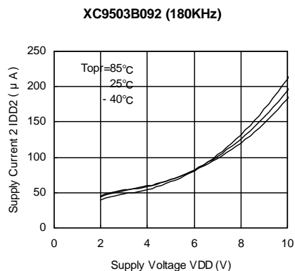
(7) Supply Current 2 vs. Supply Voltage
