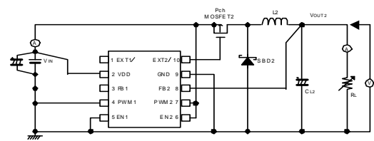
Circuit
