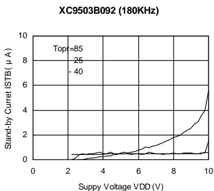
(8) Stand-by Current vs. Supply Voltage
