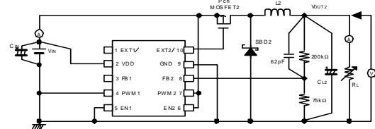
Circuit
