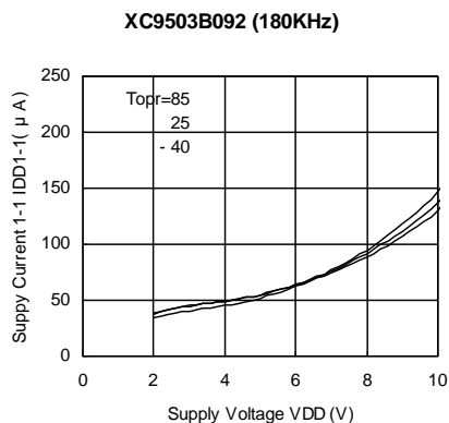
(5) Supply Current 1_1 vs. Supply Voltage
