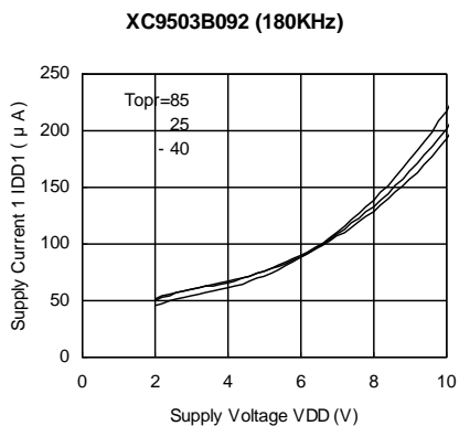
(4) Supply Current 1 vs. Supply Voltage
