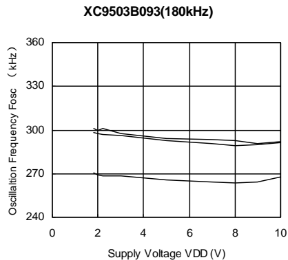
(9) Oscillation Frequency vs. Supply Voltage
