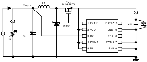
Circuit
