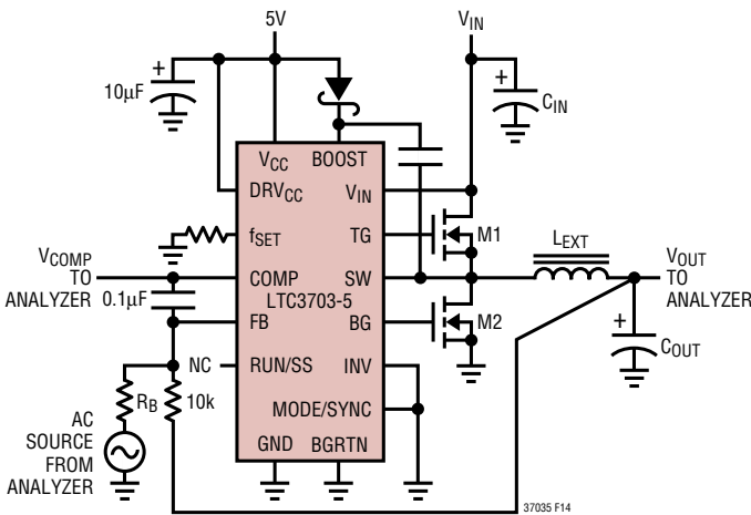
Figure 14. Modulator Gain/Phase Measurement Set-up
