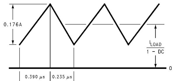
10 µH Inductor Current, 5V–12V Boost (LM2731X)
