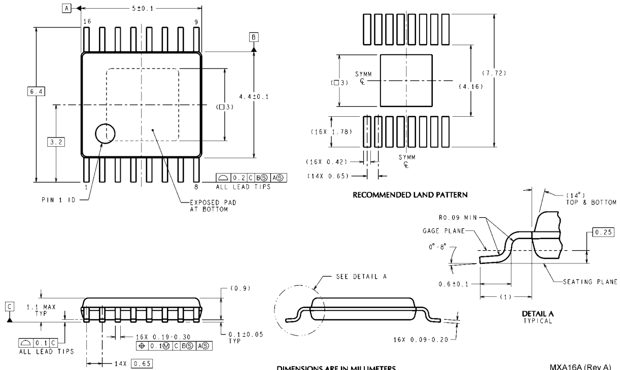
16-Lead Exposed Pad TSSOP Package NS Package Number MXA16A
