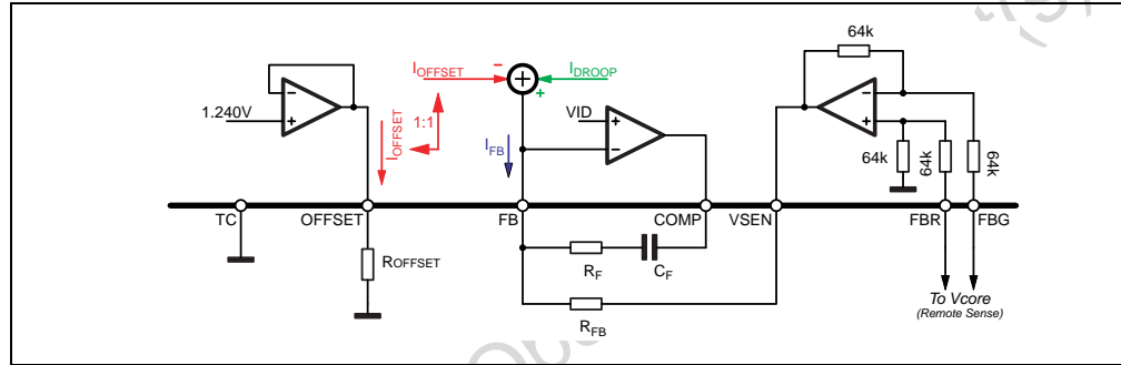
Figure 10. Voltage positioning with offset
