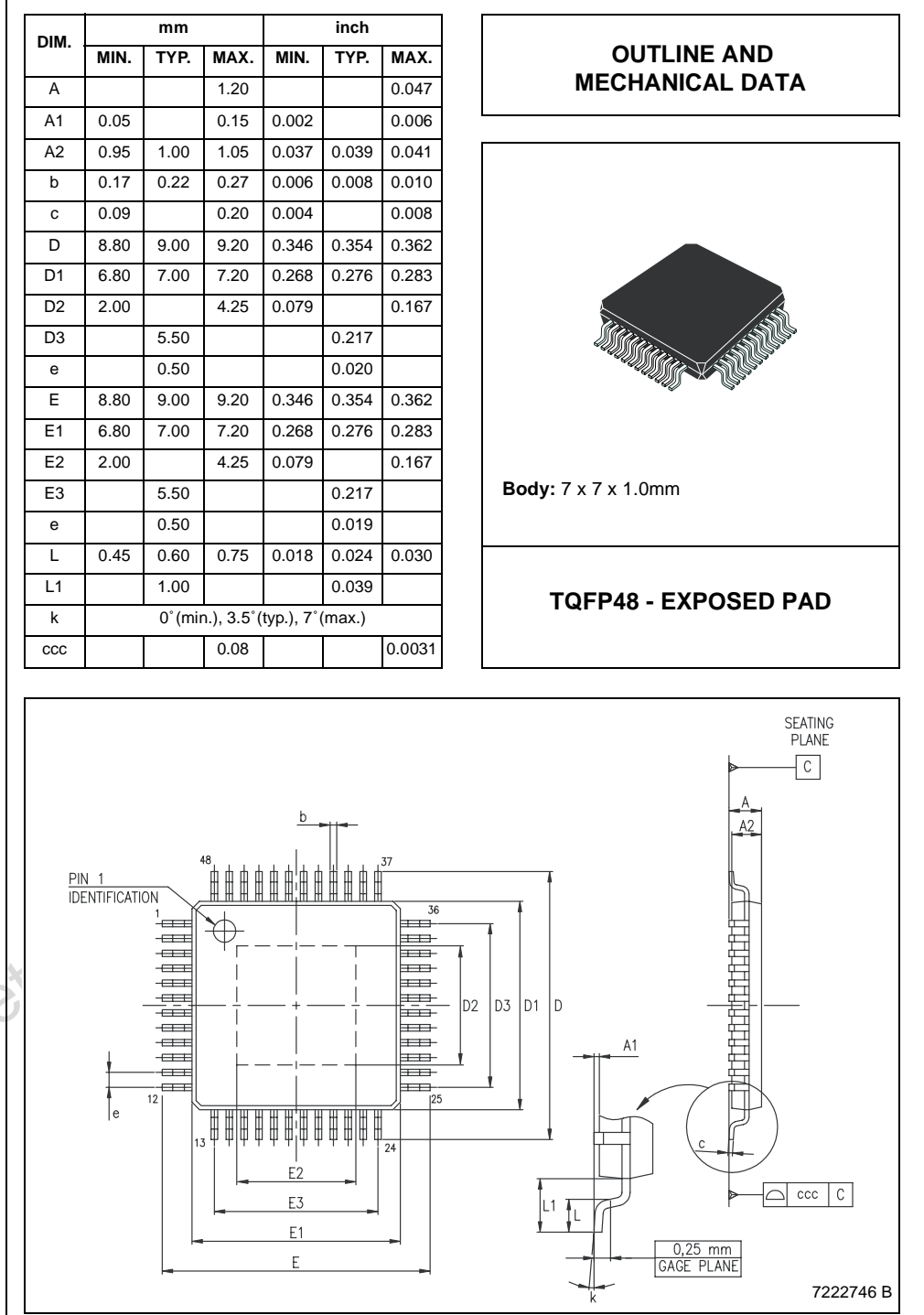
Figure 25. TQFP48 Mechanical data &amp; package dimensions
