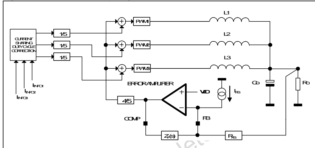
Figure 21. Main control loop diagram
