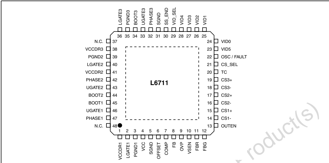
Figure 4. Pins connection (top view)
