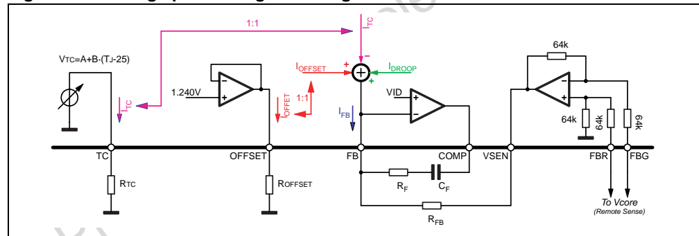
Figure 11. Voltage positioning with integrated thermal sensor
