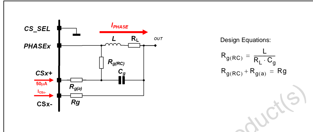
Figure 7. Inductor current sense
