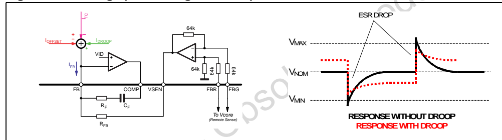
Figure 9. Voltage positioning and droop function
