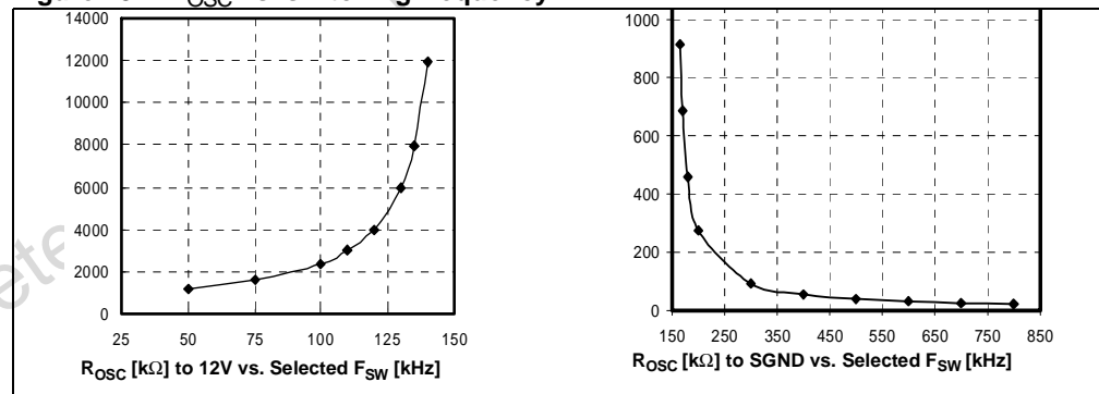
Figure 19. R_{OSC} vs. switching frequency
