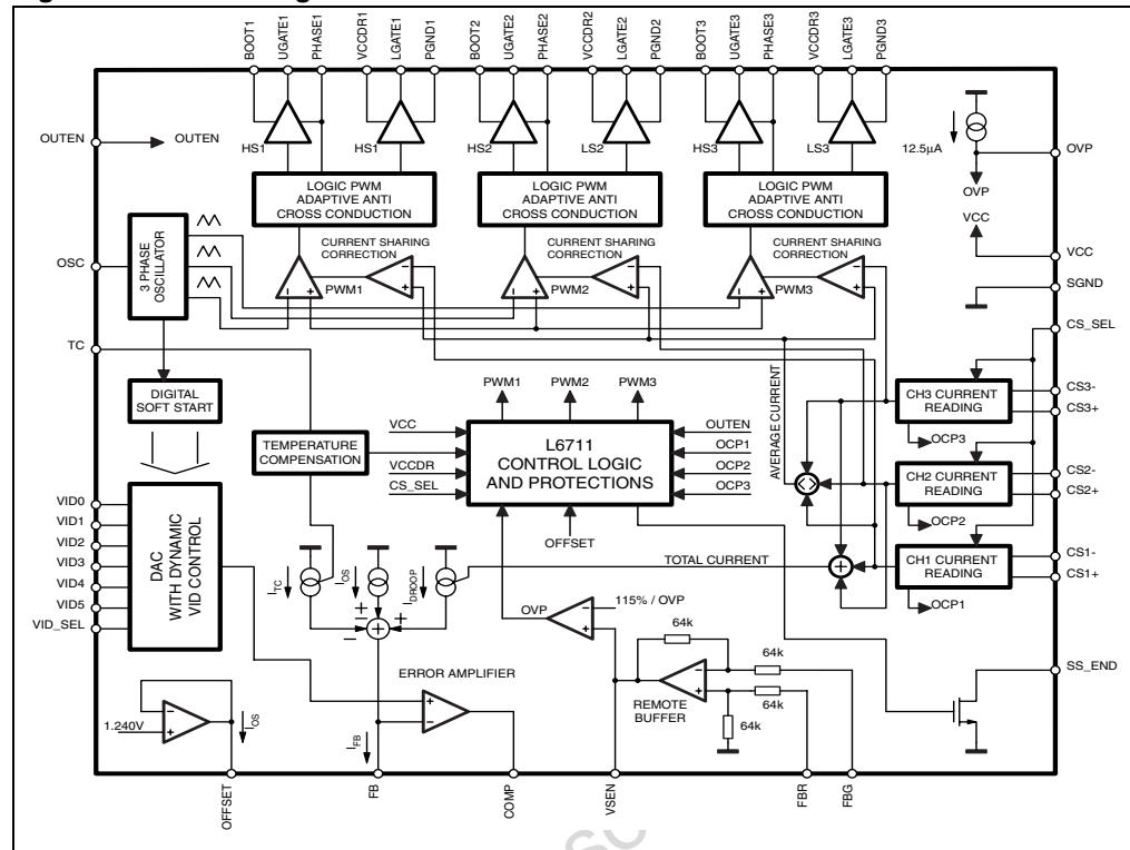
Figure 3. Block diagram
