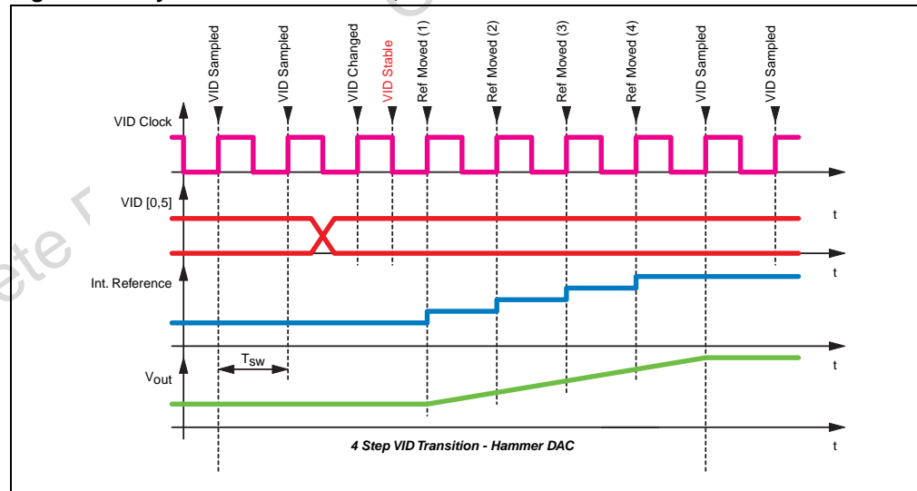
Figure 14. Dynamic VID Transition, Hammer DAC
