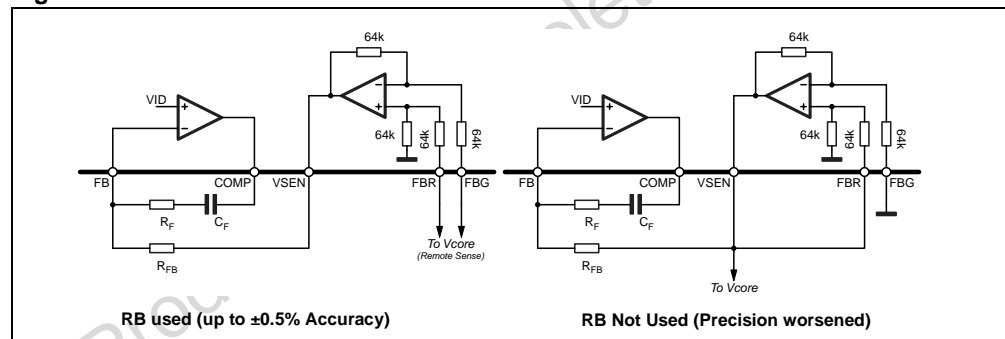
Figure 8. Remote buffer connections
