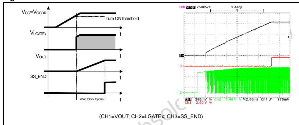
Figure 15. Soft start
