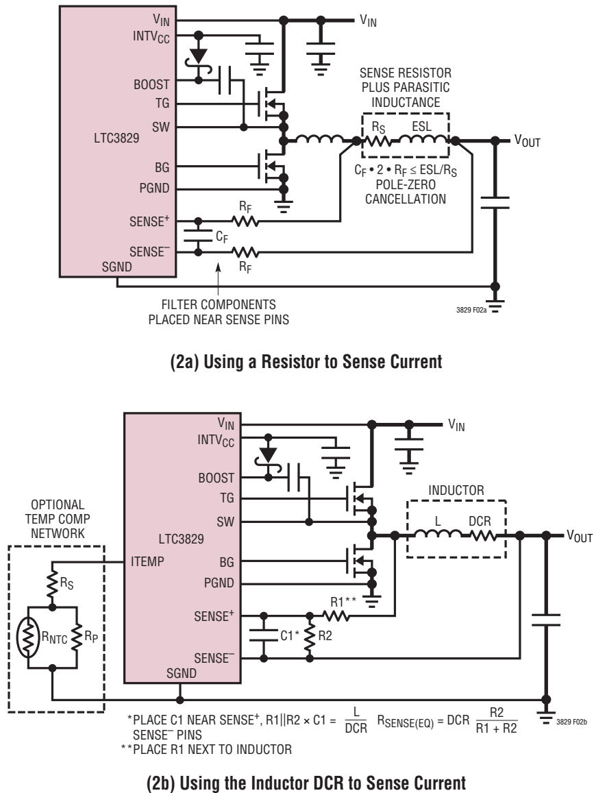
Figure 2. Two Different Methods of Sensing Current
