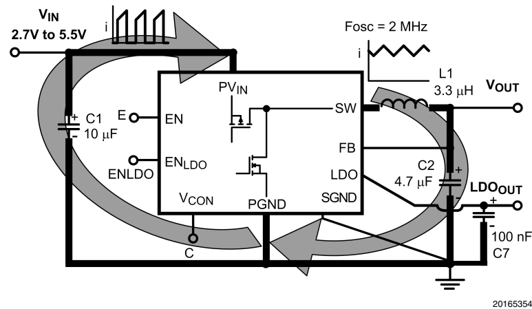
FIGURE 4. Current Loop
