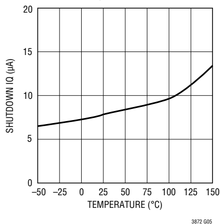
Shutdown I_{\text{Q}} vs Temperature
