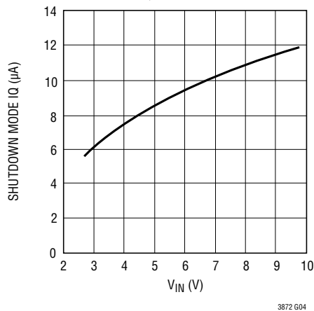
Shutdown I_{\text{Q}} vs V_{\text{IN}}
