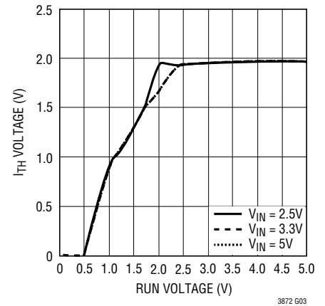
I_{\text{TH}} Voltage vs RUN/SS Voltage
