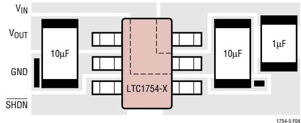
Figure 4. Recommended Layout
