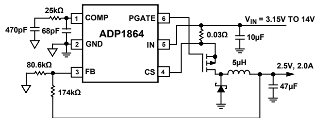
Figure 18. Application Circuit for V_{OUT} = 3.3V, 2A Load
